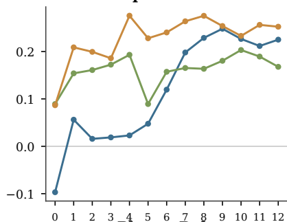
Phrase Role
