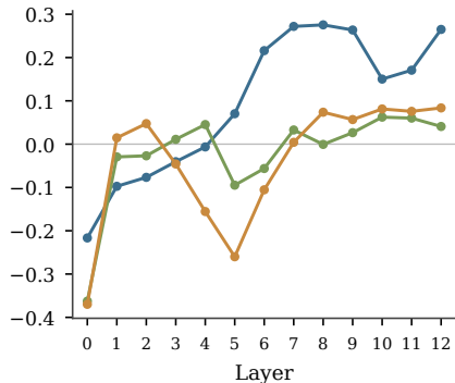
Phrase Role
